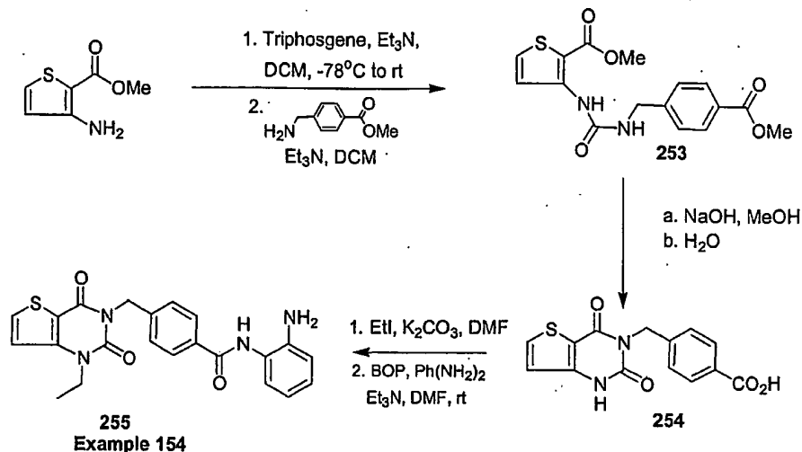
Scheme 43
